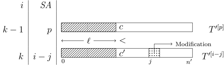
Fig. 3. T'^{[i-j]} does not have to be reordered.
