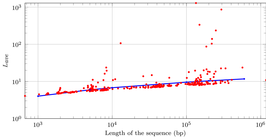
Fig. 9. L_{ave} for virus genome sequences
