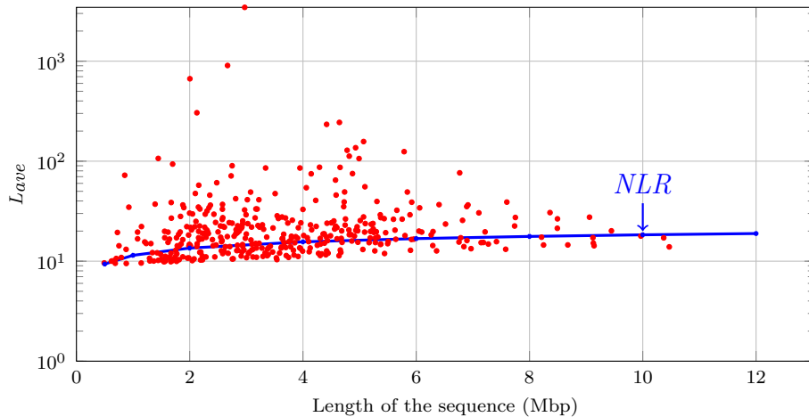
Fig. 7. L_{ave} for bacteria genome sequences
