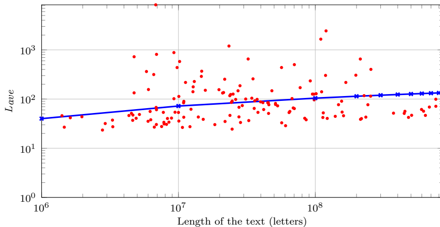
Fig. 11. L_{ave} for Wikipedia corpora
